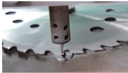
↑ Tip brazing durability test
